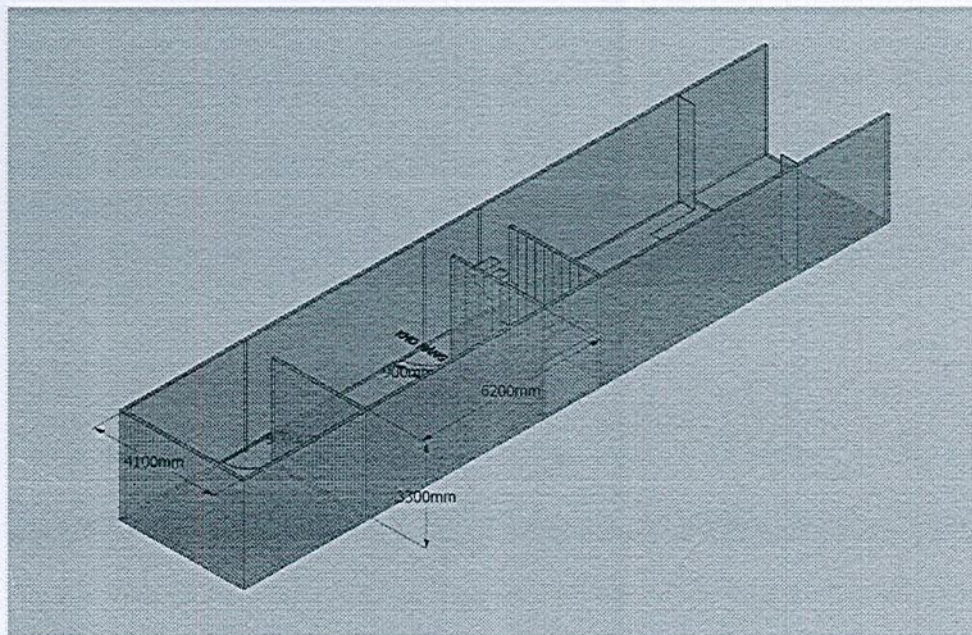
BAN DUNG 3D
